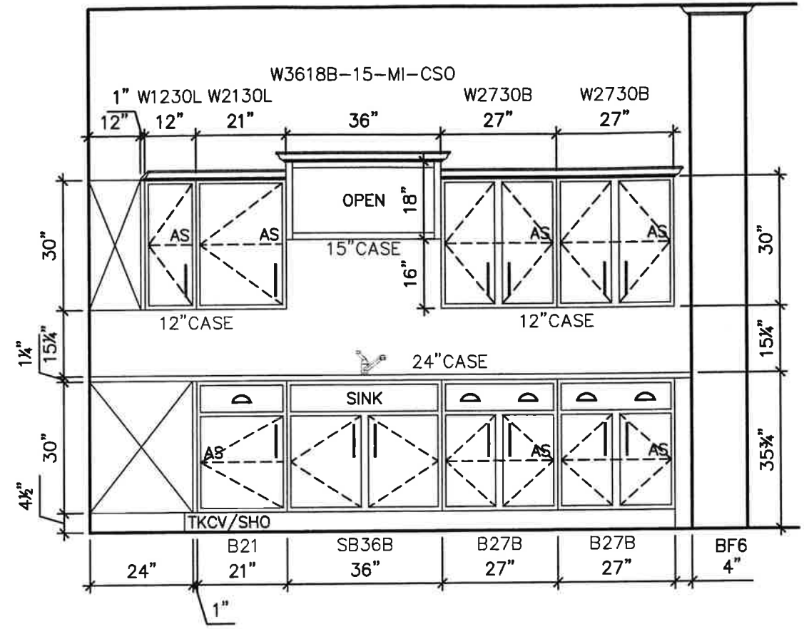
2 A021 - KITCHEN - ELEVATION VIEW 1 A105
